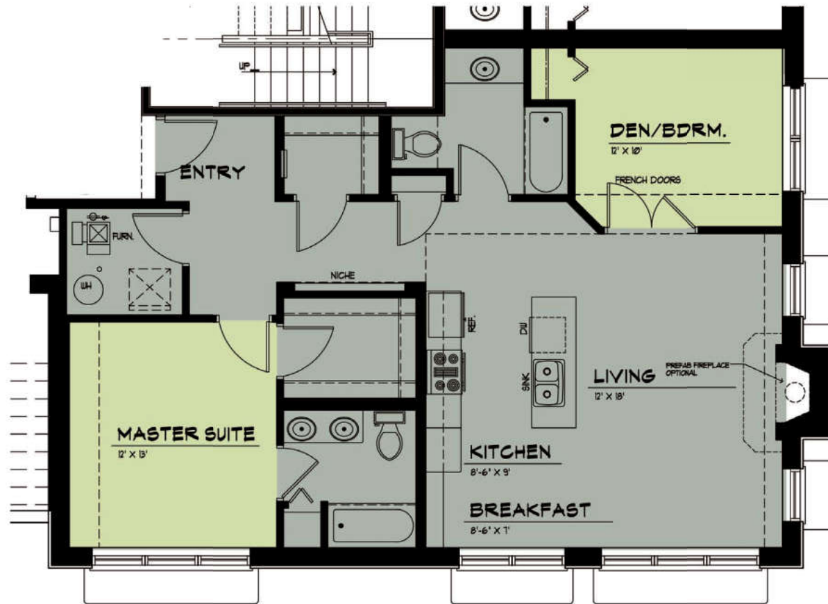
FLOOR PLAN UNIT GARDEN O2 1063 SF MULTI-FAMILY URBAN DEVELOPMENT VALPARAISO, INDIANA
