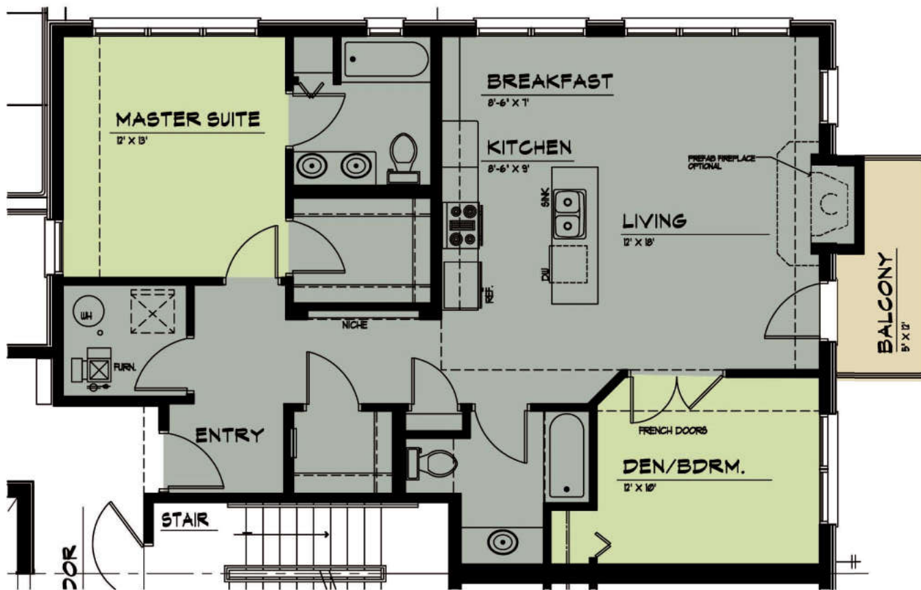
FLOOR PLAN UNIT 101, 1063 SF MULTI-FAMILY URBAN DEVELOPMENT VALPARAISO, INDIANA
